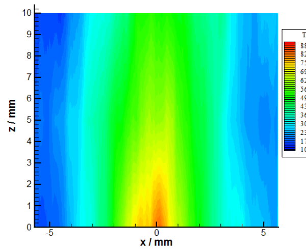
Fig. 3. Tracking accuracy of ultrafine wire
