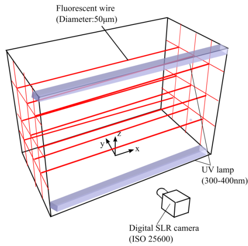
Fig. 1. Experimental setup
