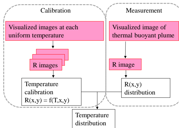
Fig. 2. Flowchart for measuring temperature
